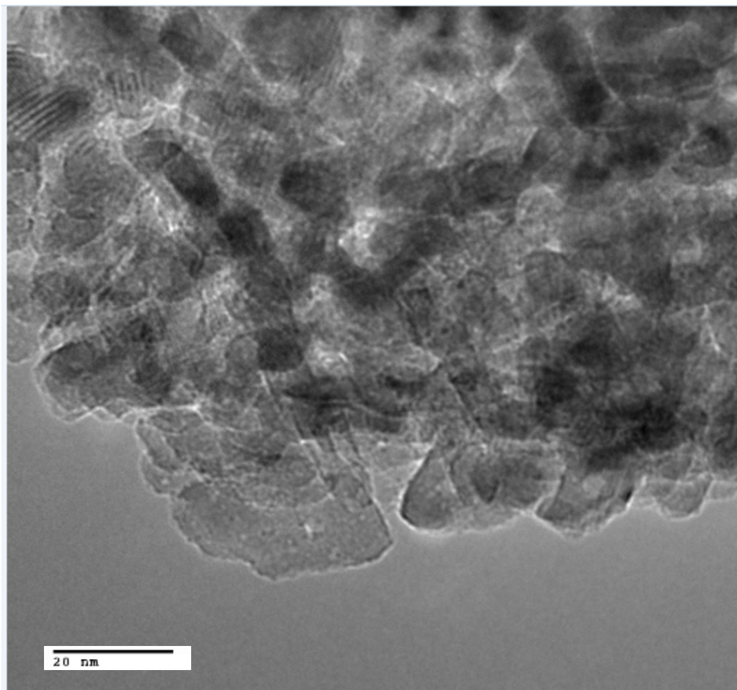
Fig S1: TEM image of RuTi400 samples pre-reduced at 400°C for one hour before imaging.
