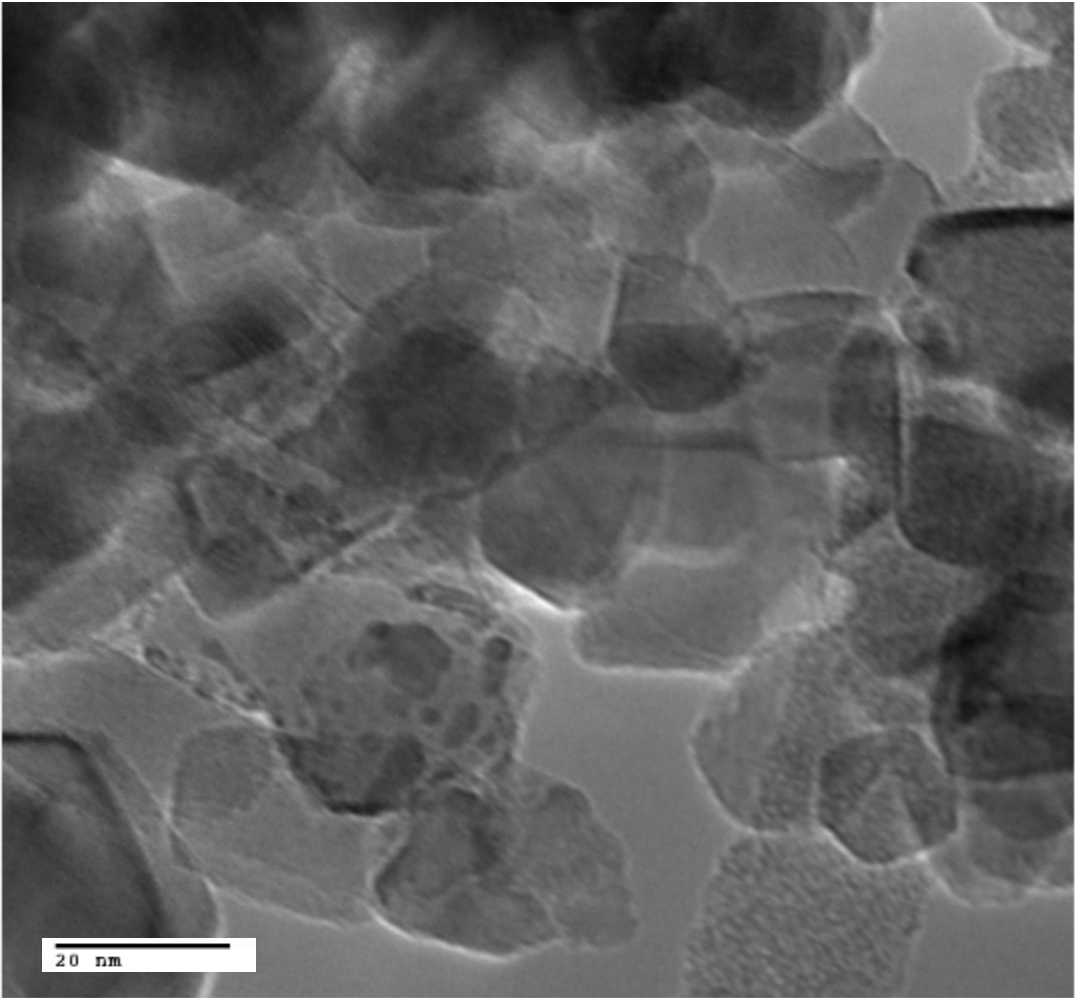
Fig S3: TEM image of RuTiP500 samples pre-reduced at 400°C for one hour before imaging.
