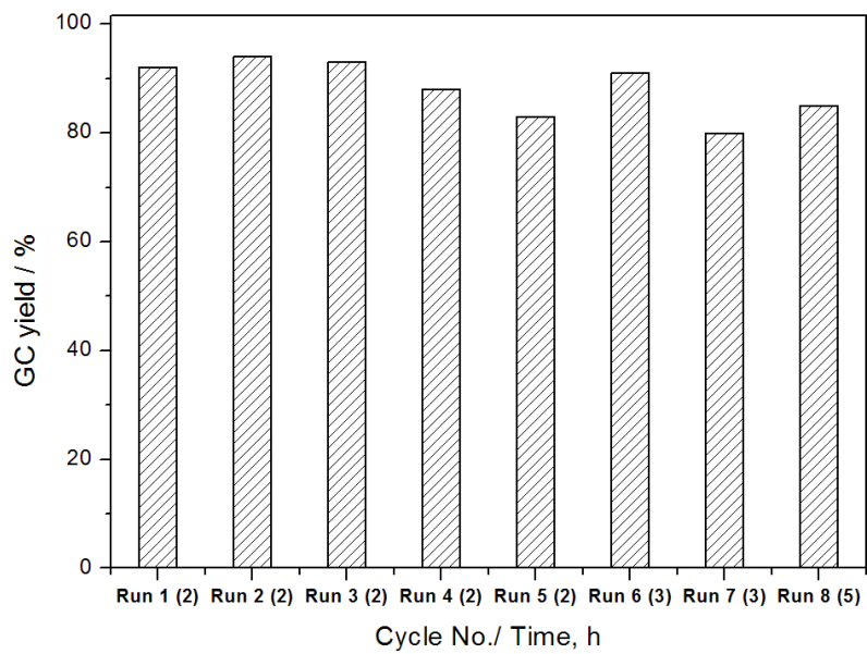
Figure S3. Recyclability of Au catalyst in the oxidation of benzyl alcohol
