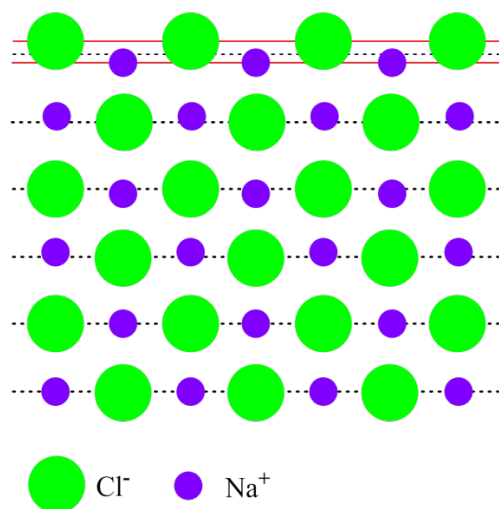
Figure S1. Schematic diagram of electric double layer on NaCl crystal surface.
