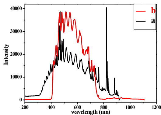
Fig.S1 The spectrum of Xenon lamp(a)and with a filter(b);
