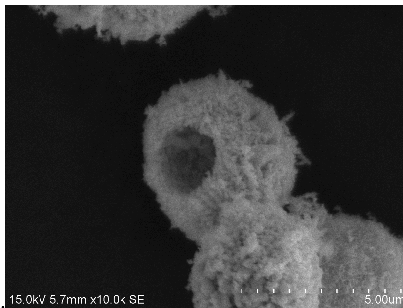
Fig. S2 SEM image of the resulting graphitized carbon after composites of \text{HNO}_3 and \text{H}_2\text{O}_2 were hired to remove the \text{Bi}_2\text{WO}_6@\text{CeO}_2 .
