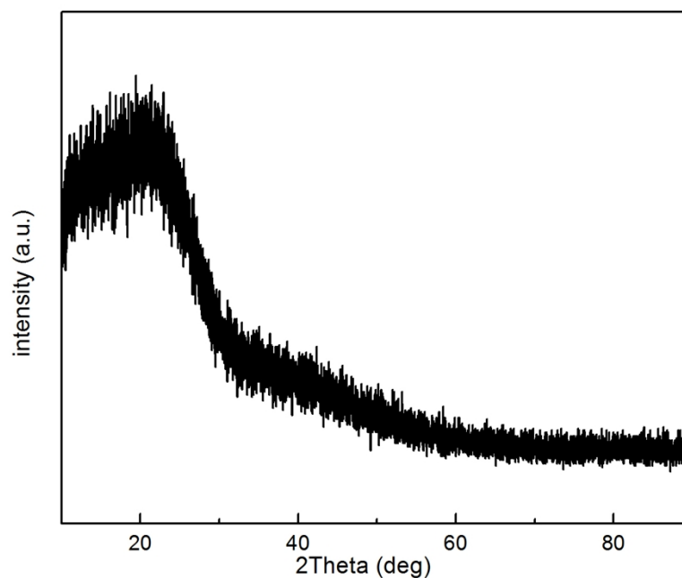
Fig. S1 XRD of the resulting graphitize carbon after composites of \text{HNO}_3 and \text{H}_2\text{O}_2 were hired to 5 remove the \text{Bi}_2\text{WO}_6@\text{CeO}_2 .
