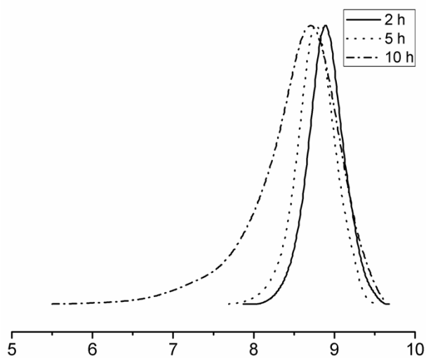
Fig. S2 GPC analysis of PVAc-Br.
