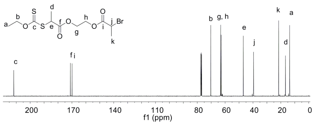
Fig. S1 13 C NMR analysis (CDCl 3 ) of S -[1-Methyl-4-(6-Bromopropionate) Ethyl Acetate] O -Ethyl Dithiocarbonate.
