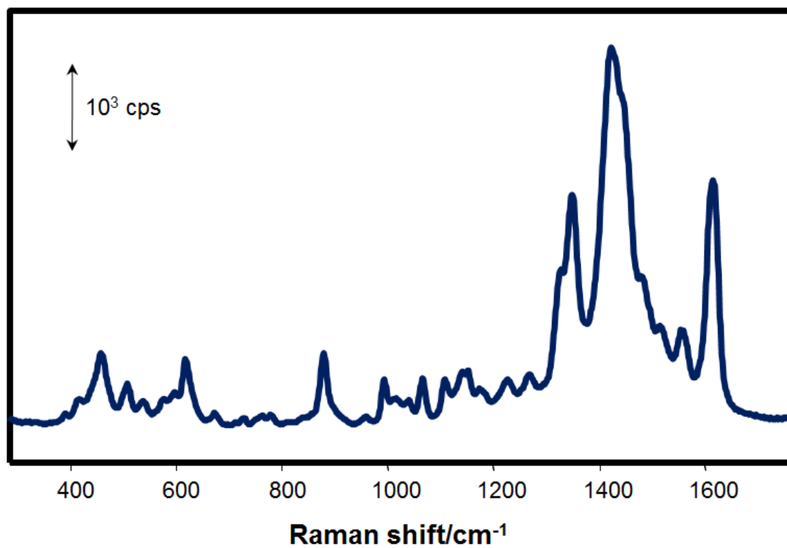
Figure S1. SERS spectrum of the TB encoded nanospheres upon excitation with a red laser (633 nm).
