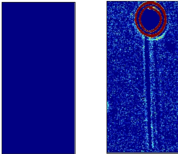
Movie S3. Two 40 \mu\text{m} micron tubes formed from mast cell of mouse in presence of cytochalasin E. Left panel: Relaxation, 25.0 s of data shown at 6 fps (25 x 6 frames). Right panel: Tube pull-back towards the cell when the optical trap was removed, 23.6 s of data shown at 6 fps (23.6 x 6 frames). Dimensions of image in movies are 13.8 by 28.6 \mu\text{m} .
