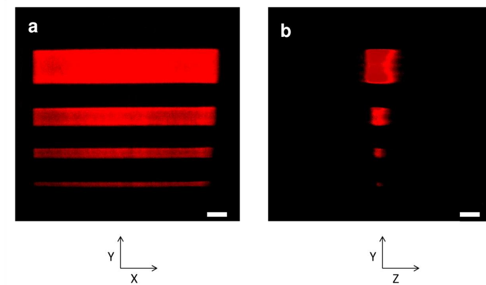
Supplementary Figure 1: 3D Patterns of PEG-RGDS Vary in Width and Height. PEG-RGDS micropatterns within a PEG-PQ hydrogel are shown. (a) Straight on (XY) view of micropatterns showing a constant 500 \mu\text{m} length and various widths of 100, 50, 25, and 10 \mu\text{m} . (b) Cross sectional (YZ) view of micropatterns showing that the patterns have controlled widths and heights. From top to bottom the YZ dimensions of the patterns are 100 x 100 \mu\text{m} , 50 x 50 \mu\text{m} , 25 x 25 \mu\text{m} , and 10 x 10 \mu\text{m} . Scale bar = 50 \mu\text{m} .
