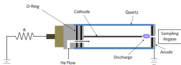
Figure S-1. Diagram of the FAPA source used in this study.
