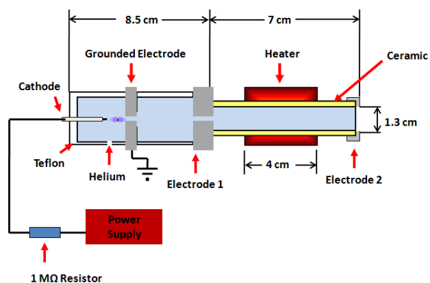
Figure S-2. Diagram of the home-built DART source used in this study.
