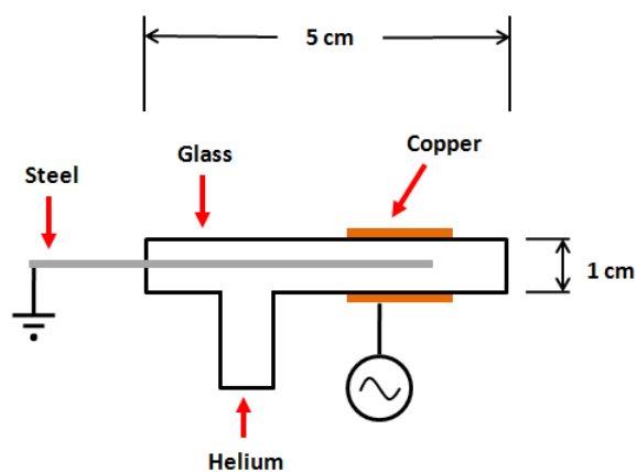
Figure S-3. Diagram of the home-built LTP source used in this study.
