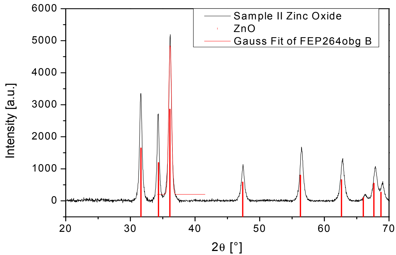
Figure S1. XRD of insitu prepared ZnO
