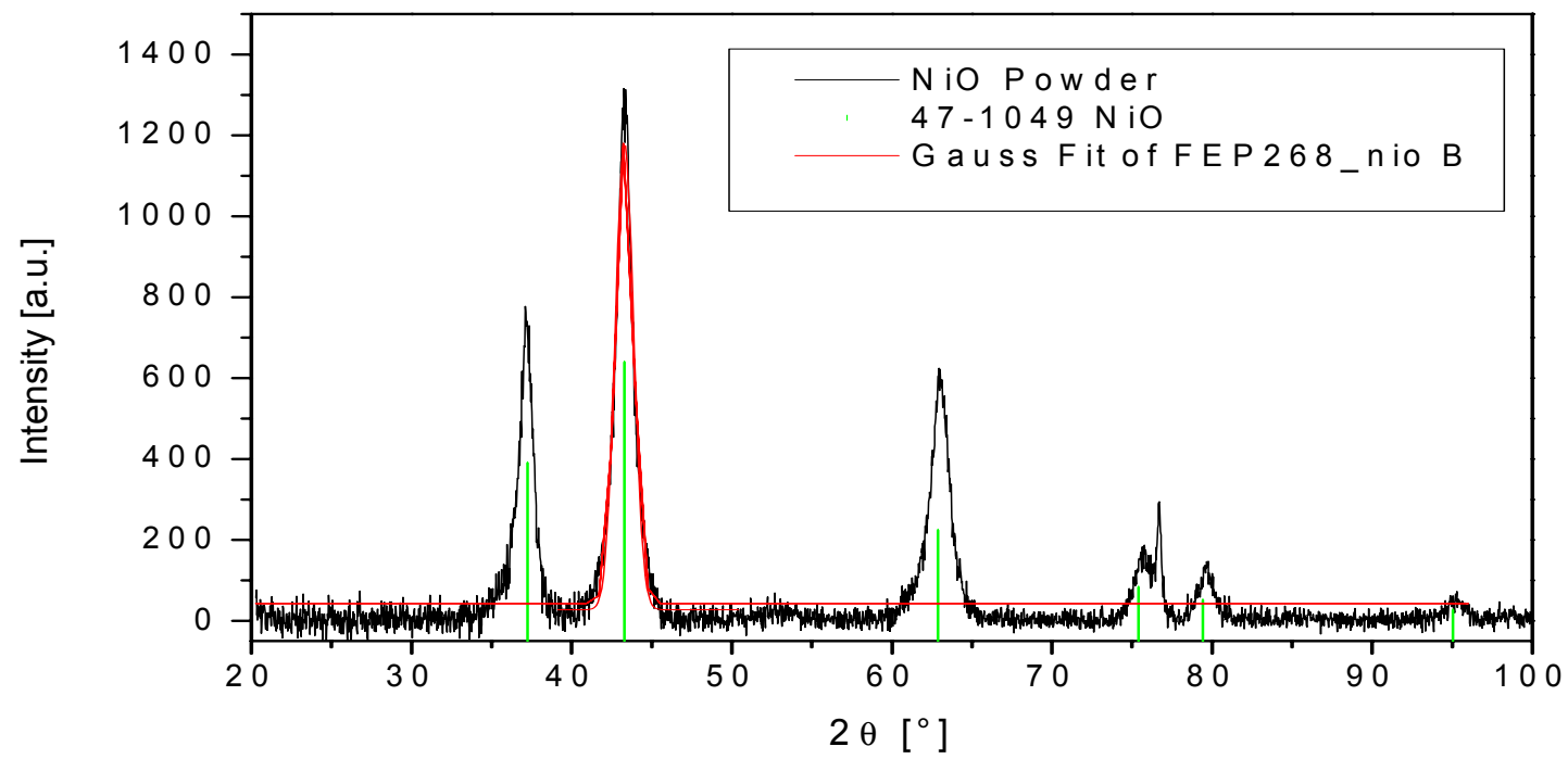
Figure S2. XRD of insitu prepared NiO
