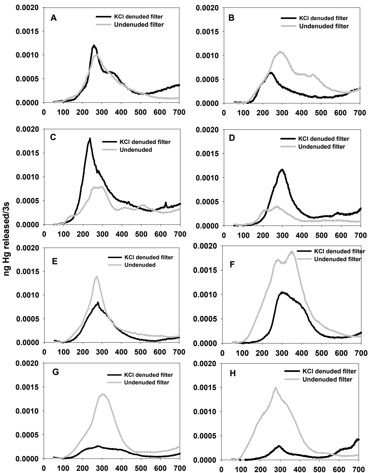
2 3 Figure S1 Mercury release, ng/3s versus temperature, for denuded and undenuded fine particulate 4 mercury samples collected in Detroit, MI
