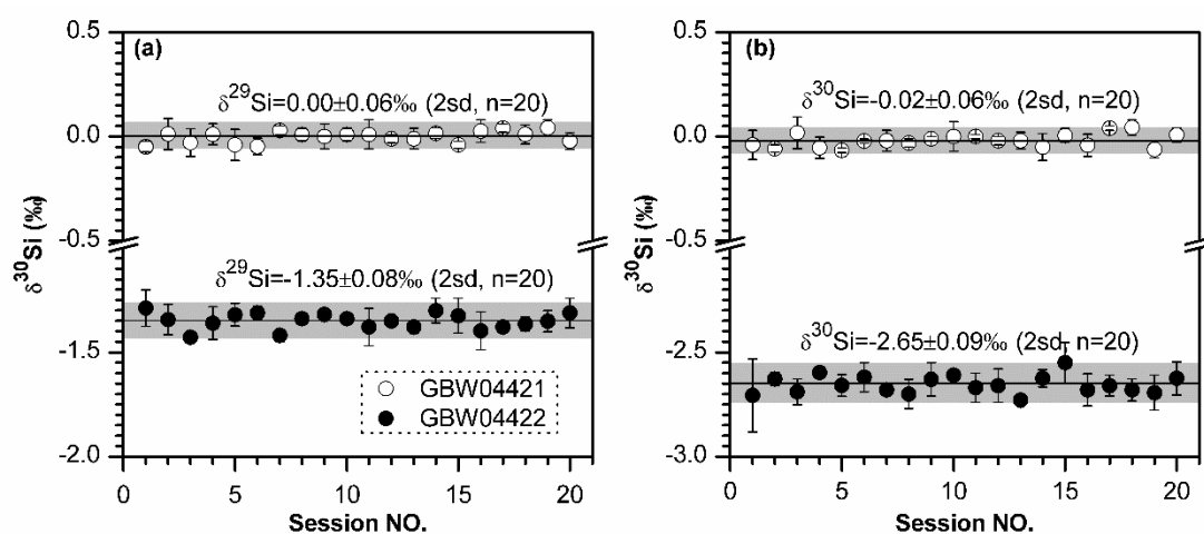
Figure S1 Long-term measurements of national Si reference materials GBW04421 and GBW04422 relative to NBS28. The solid black lines and grey shadow area denote the average value and 2 standard deviation.
