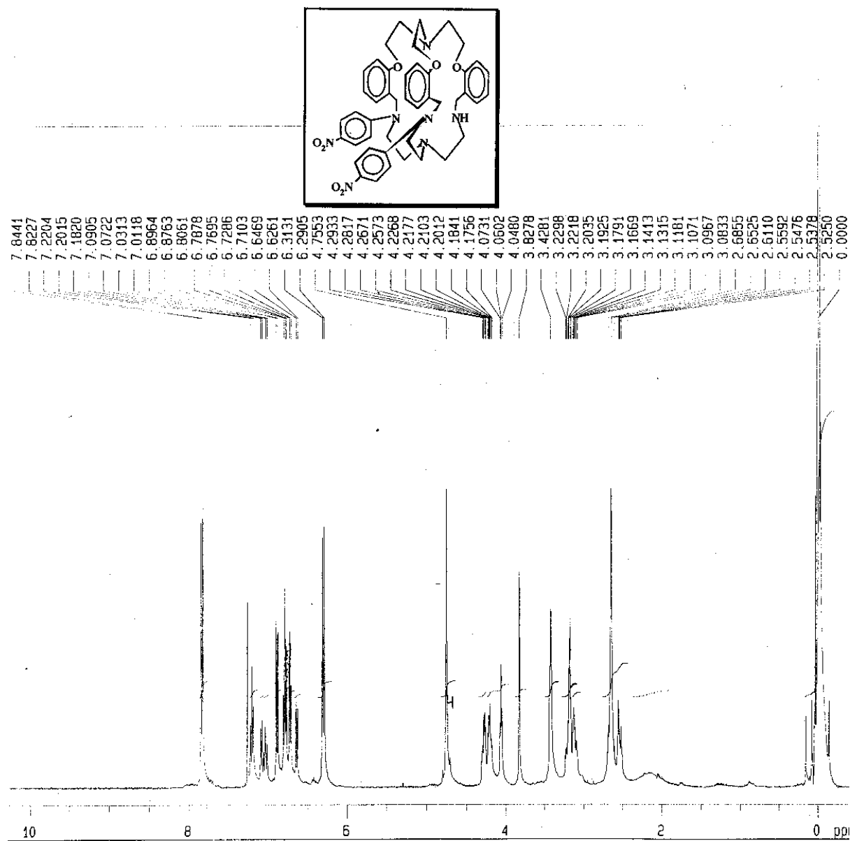
400 MHz 1 H-NMR spectrum of compound B 3
