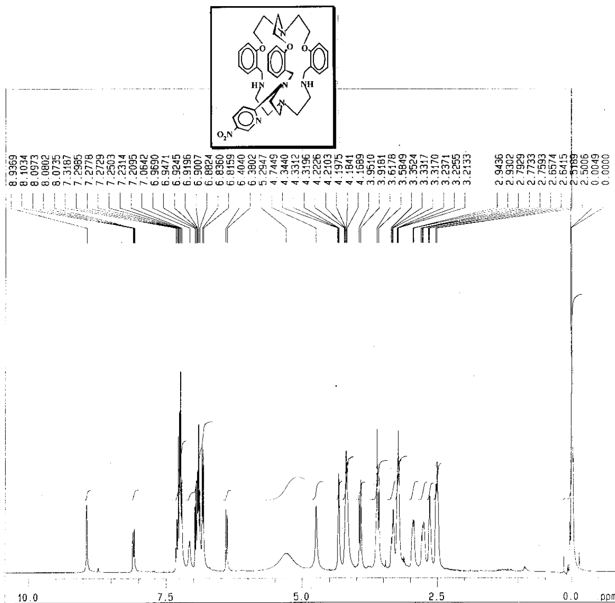
400 MHz 1 H-NMR spectrum of compound M 2
