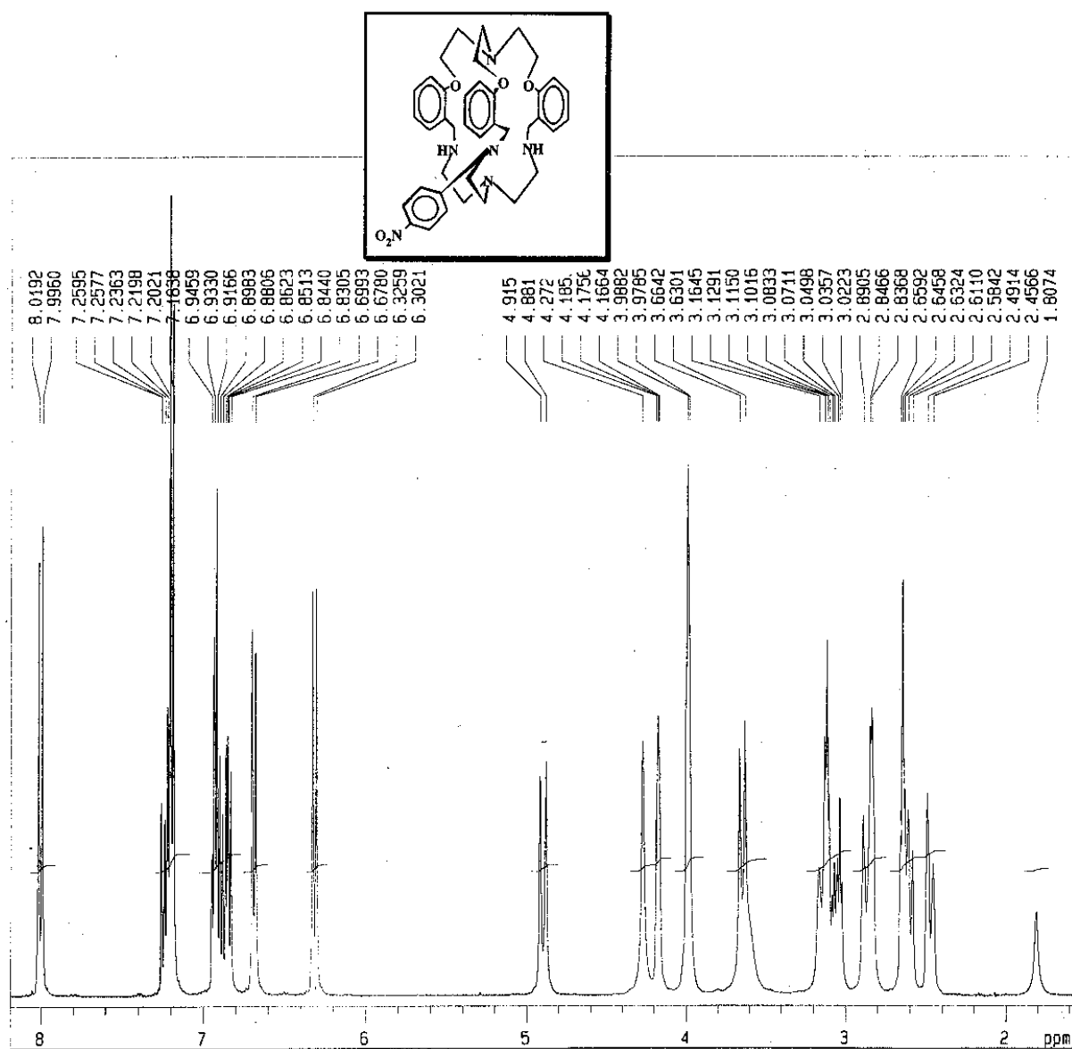
400 MHz 1 H-NMR spectrum of compound M 3
