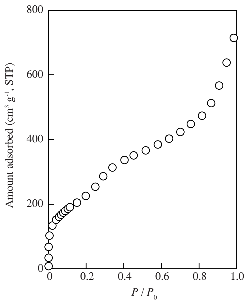
Supporting Information Figure S3 N 2 adsorption isotherm of Al-KSW-2 (0.03).
