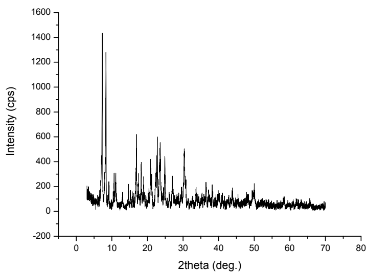
Figure S7 PXRD of M(C_4H_9NH_2)_3
