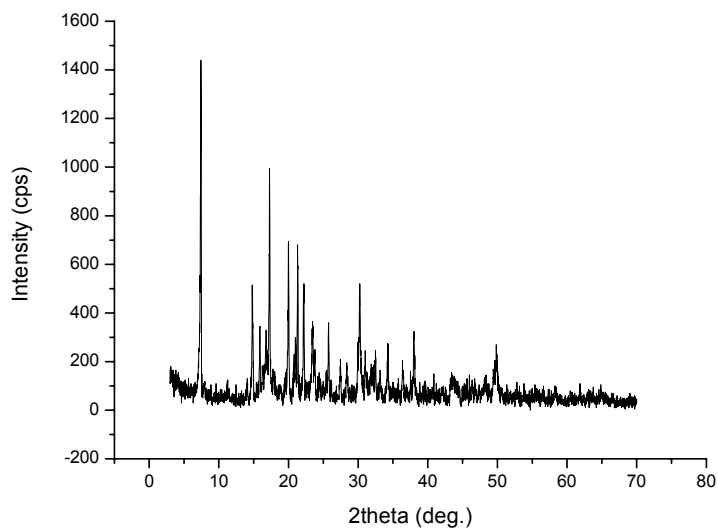
Figure S2 PXRD of M(NH 3 ) 3
