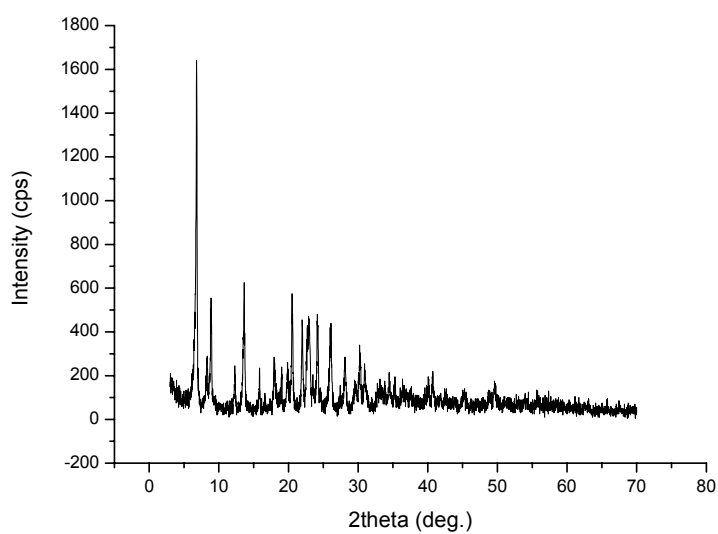
Figure S10 PXRD of M(C_8H_{17}NH_2)_2
