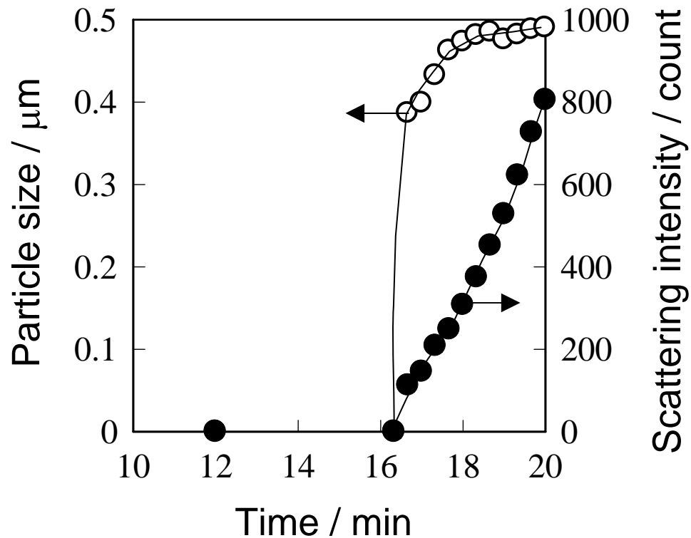
ESI. Time courses of particle size and scattering intensity of the sample synthesized with TEOS and C_{16} TMACl.
