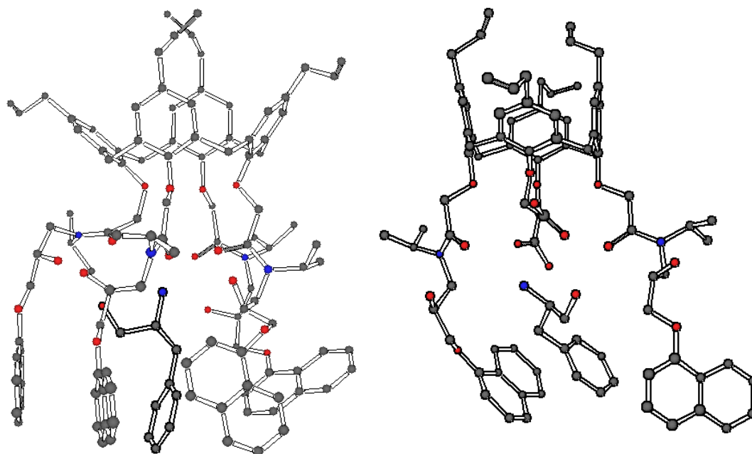
Figure 9: Side-on view of L1 and PA (left of picture) and L2 and PA (right of picture), showing how the guest may be included in the calixarene cavity, and also the extent of steric crowding involved. The modelling calculations were carried out using Spartan [i] SGI Version 5.1.1. The models shown correspond to the conformer found with the lowest energy
