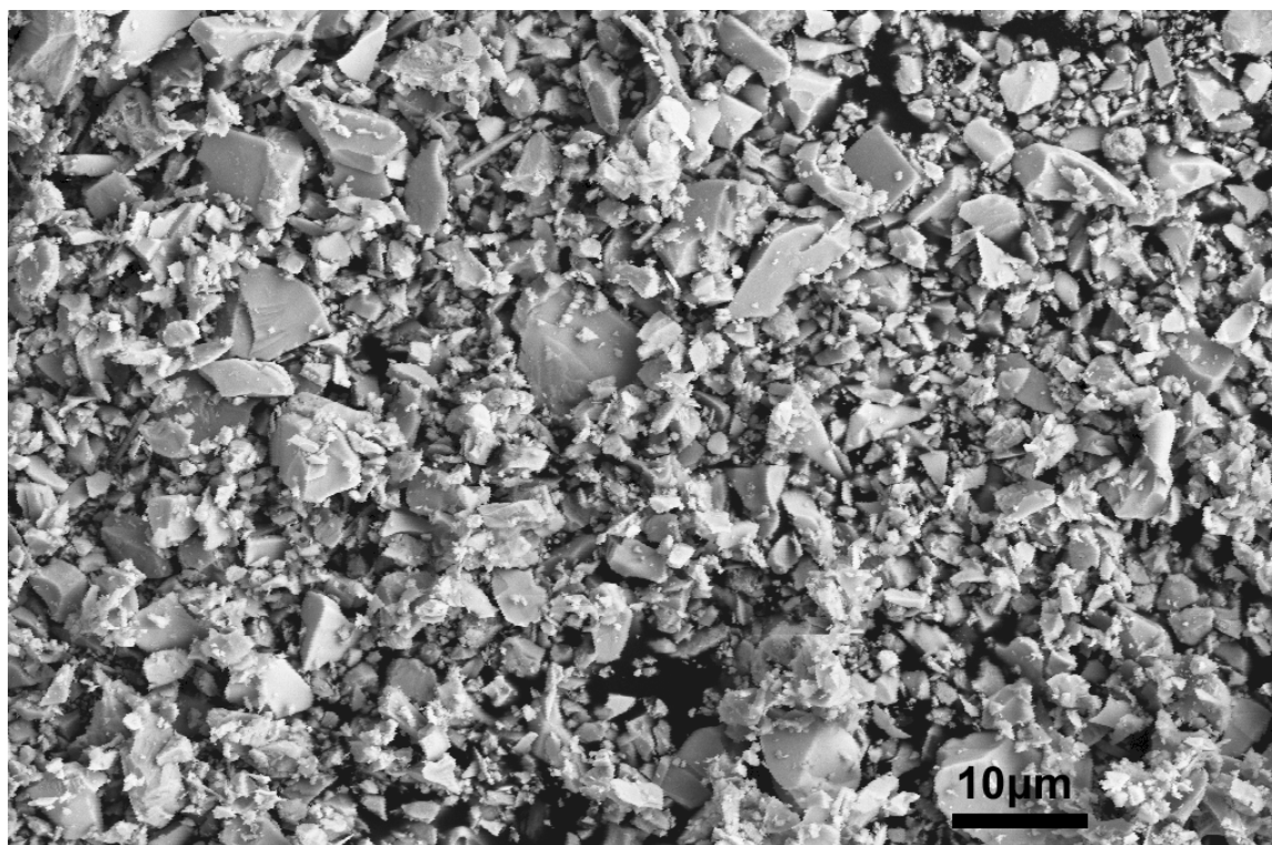
Figure S1. SEM image of Bi 2 Fe 4 O 9 materials prepared using the method described herein but in the absence of NaCl.
