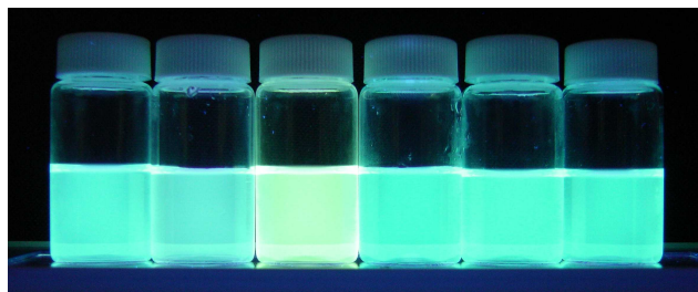
ESI-Fig 1 Acetonitrile solutions of 10 \mu\text{M} CDP 10 in the presence of 5 mM metal ions. The excitation is by a UV lamp set at 360 nm. The metal ions from left to right are; Zn(II), Mg(II), Ca(II), K(I), Na(I) and Li(I).
