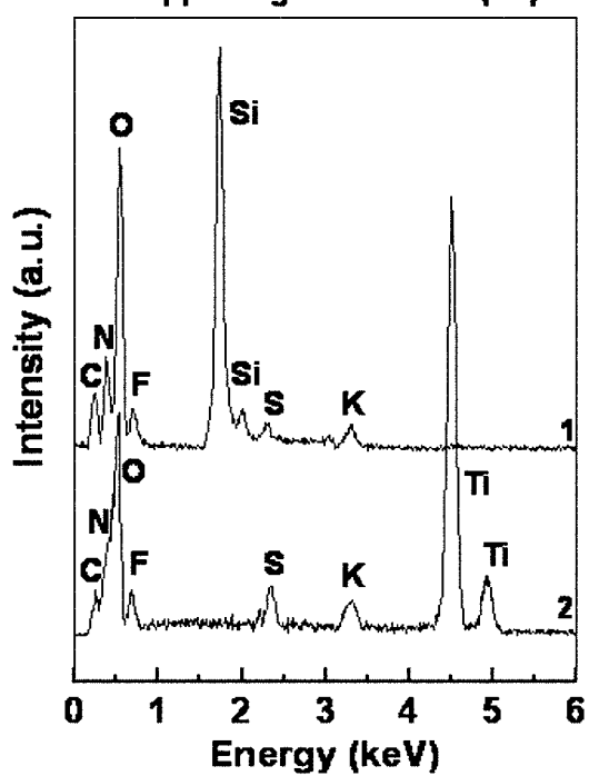
S1. EDAX spectra recorded from biogenic silica (curve 1) and titania (curve 2) particles synthesized using the fungus, Fusarium oxysporum .
