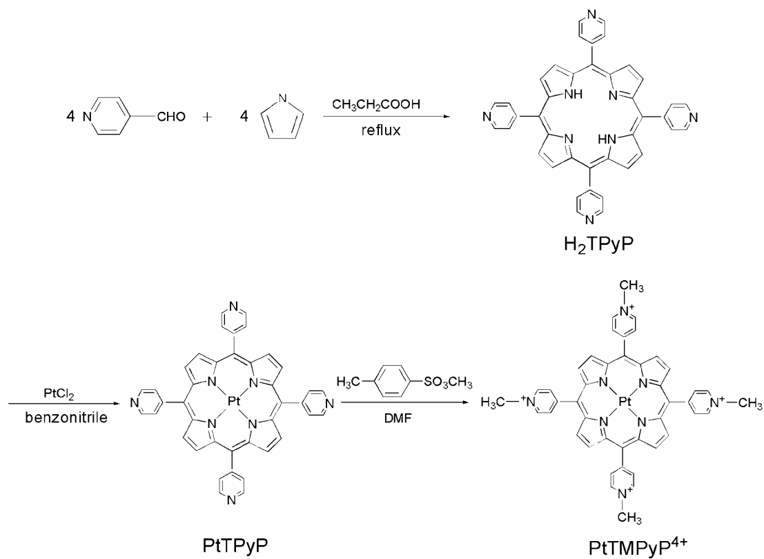
The synthesis scheme of Pt(II)-porphyrins
