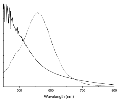
Figure S2: Extended absorption (—) and photoluminescence (---) spectra of representative smaller CdSe nanocrystals in cyclohexanone.
