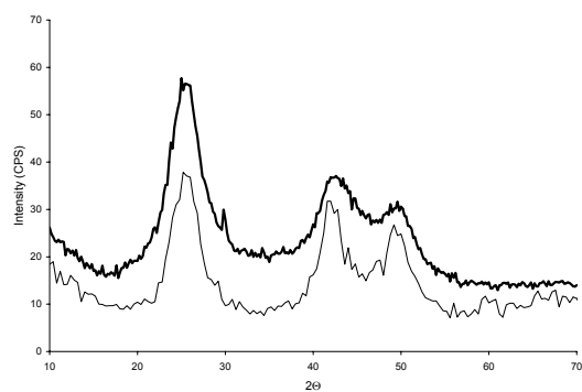
Figure S3. X-ray powder pattern of representative small (—) and larger (---) CdSe nanocrystals
