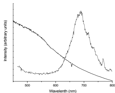
Figure S1: Extended absorption (—) and photoluminescence (---) spectra of representative larger CdSe nanocrystals in cyclohexanone.
