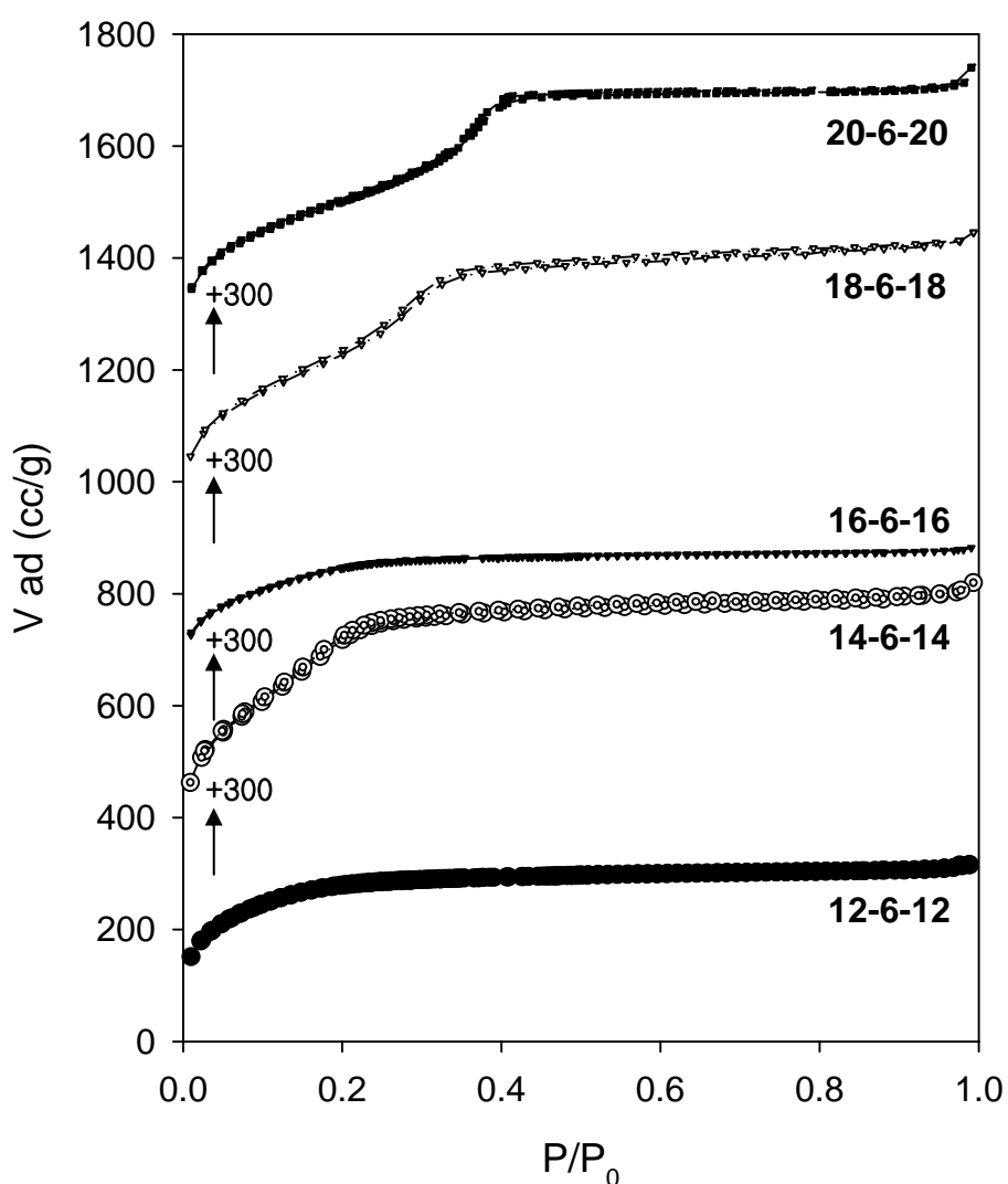
Figure S1 Nitrogen adsorption-desorption isotherms for the PMO materials in Fig. 1.
