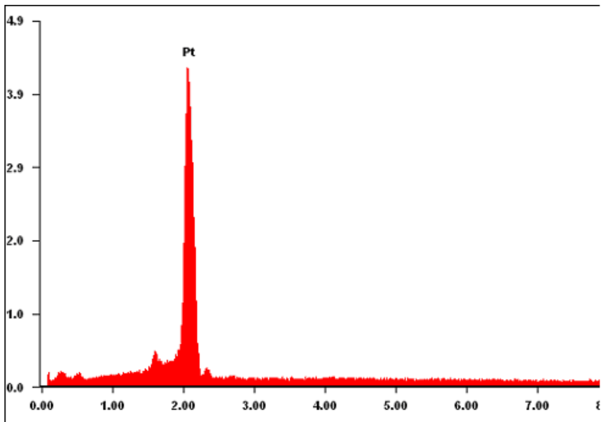
EDX spectrum of the Pt nanoparticles.
