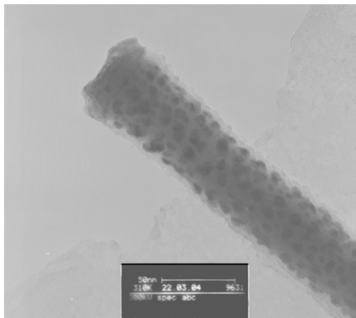
Figure S1: TEM image of PbS nanoparticles within the matrix of nanowire grown at 700 °C on substrate 1.
