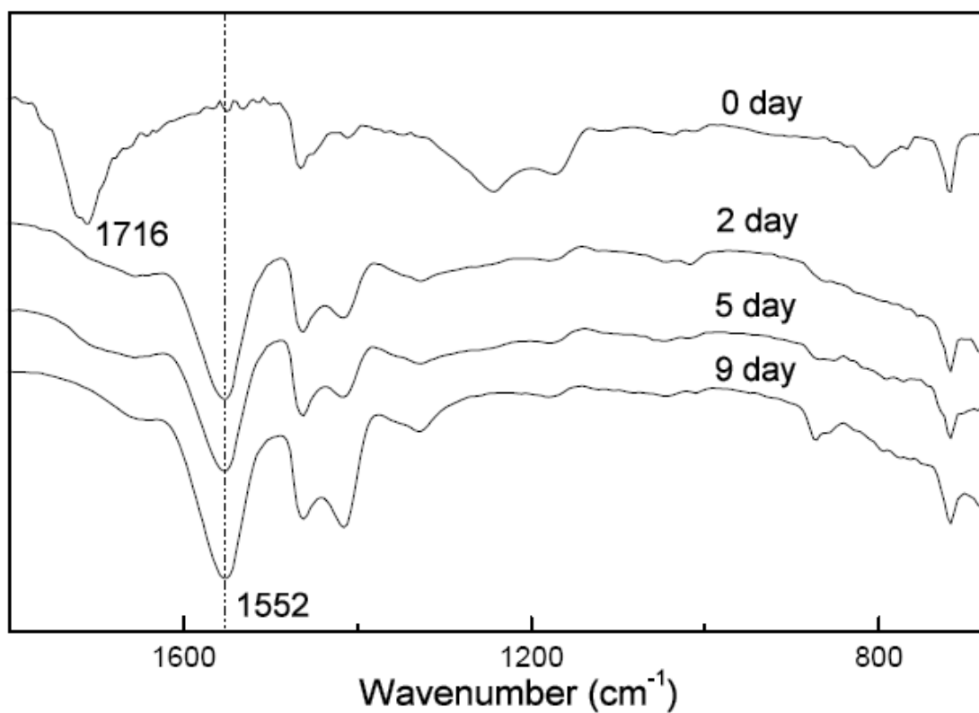
Fig.S1. ATR-IR spectra of grafted PE substrates (degree of grafting is about 50%) soaked in supersaturated calcium bicarbonate solution for different periods of time.
