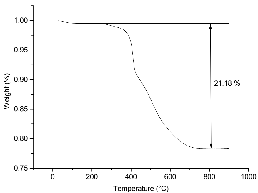
Fig S1. Thermogravimetric analysis of 'as-made' [F, Tet-A]-AlPO-1. Heating rate of 10^{\circ}\text{C min}^{-1} in flowing oxygen.
