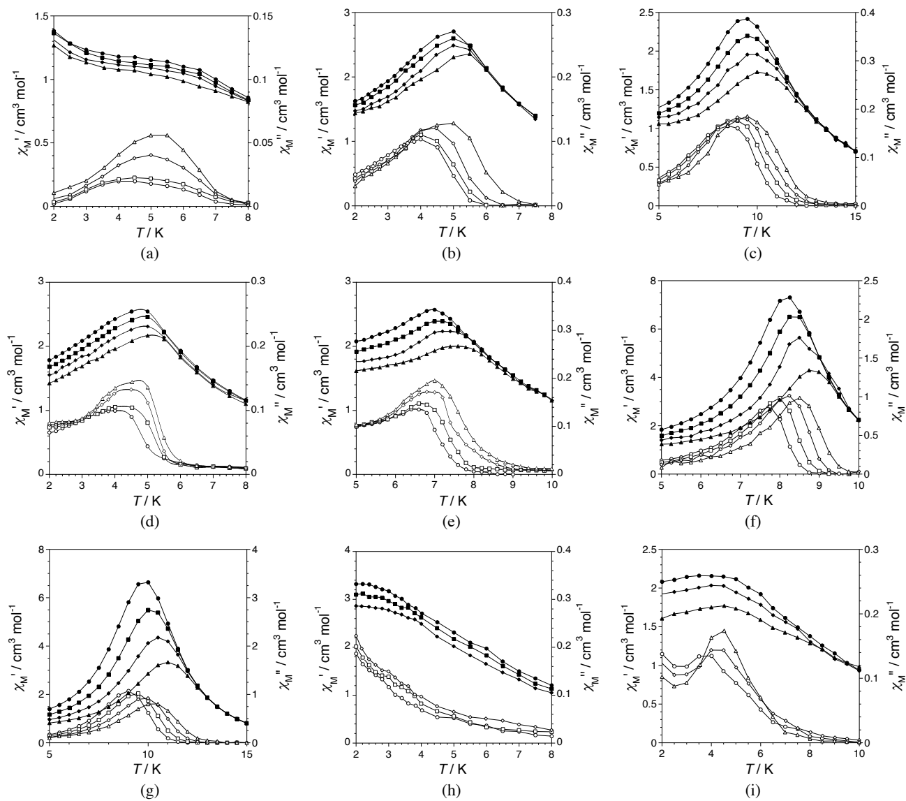
Fig. S1 Temperature dependence of \chi_M' and \chi_M'' (open symbols) for IA–I (a)–(i) in zero DC field and under 1G AC field at oscillating frequencies of 1 (●), 10 (■), 100 (◆), and 1000 Hz (▲). The solid lines are eye-guides.
