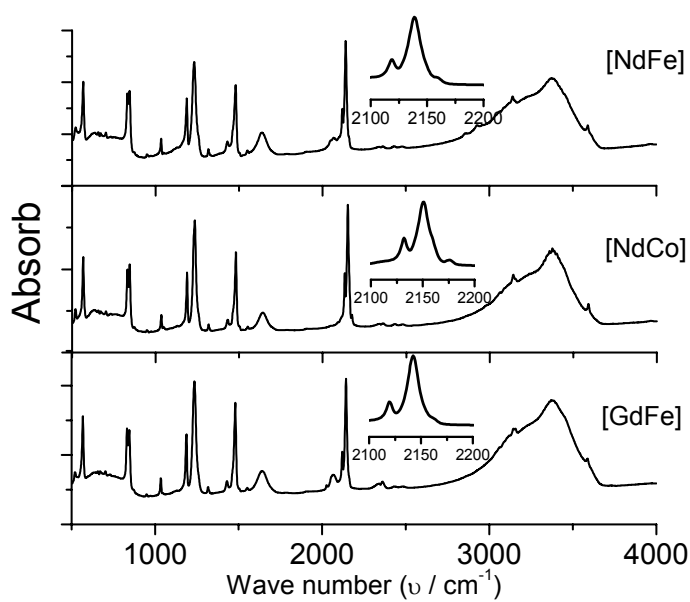
Fig. S1 IR spectra for compounds 1-6
