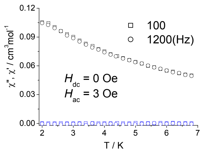
Fig. S2 Real ( \chi_M' , upper) and imaginary ( \chi_M'' , down) ac susceptibilities in zero static applied field and an ac field of 3 Oe at different frequencies for 5 .
