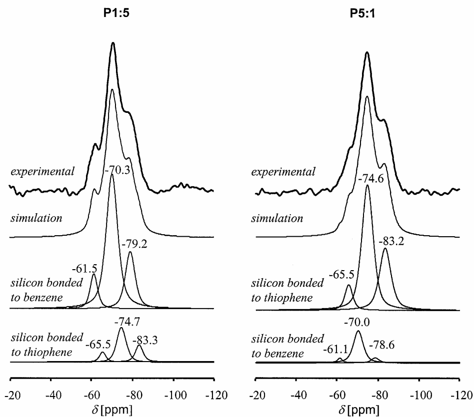
Figure S1: Simulation of the ^{29}\text{Si} MAS NMR spectra of the bifunctional PMO materials P1:5 (left) and P5:1 (right) according to Figure 7.
