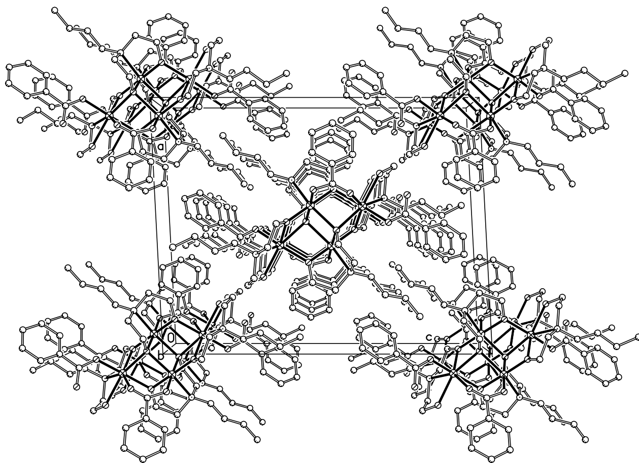
Packing diagram (viewed down b -axis) for complex 2
