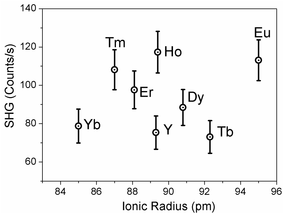
Supplementary Information 2 SHG Intensity as a function of the ionic radius of the rare-earths.
