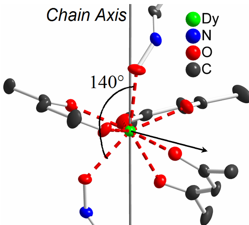
Supplementary Information 3 Coordination geometry around the rare-earth metal centre. The Radical oxygen –Metal– Radical oxygen angle is reported. The black arrow represents the direction of an hypothetical cis coordination of the radicals.
