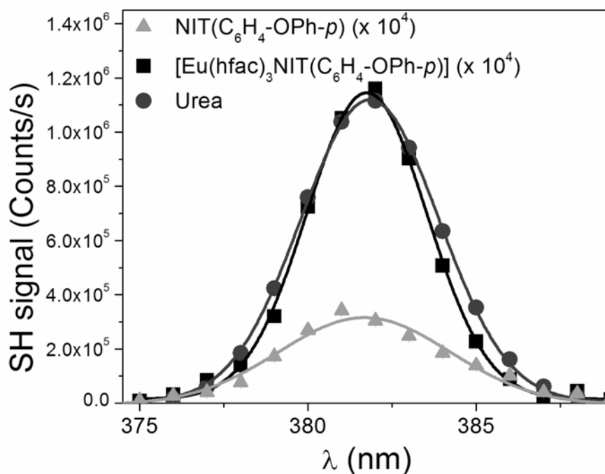
Supplementary Information 1 Spectral dispersion of the Fundamental and SHG beams
