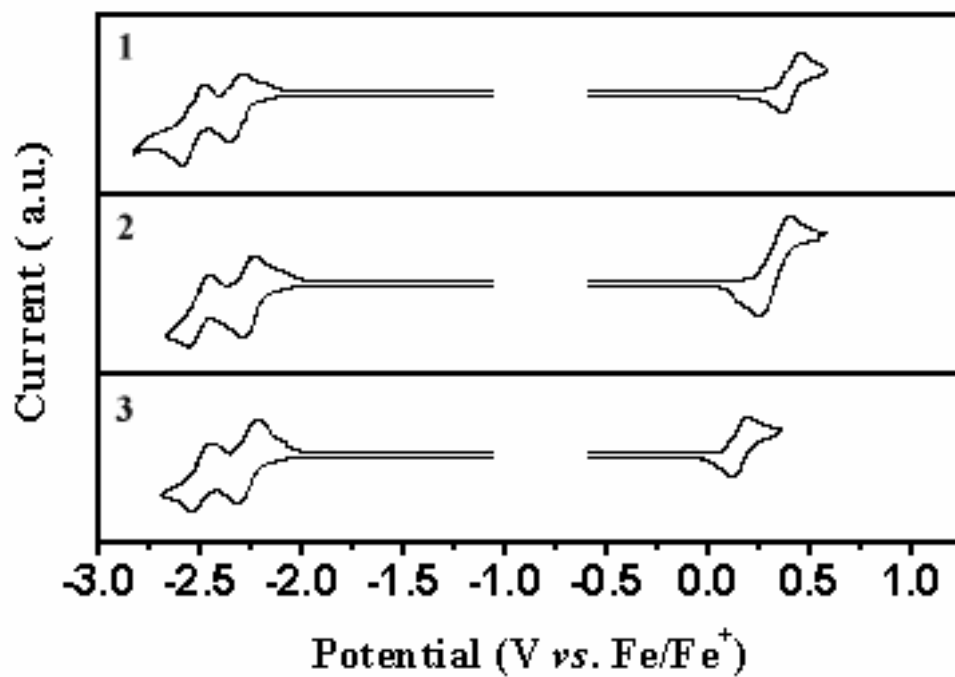
Figure S1: Representative cyclic voltammograms of complex 1, 2 and 3.
