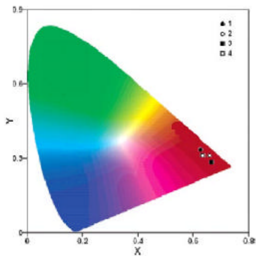
Figure S2: CIE 1931 coordinates plot for the devices using complex 1 , 2 , 3 and 4 as dopant at 3 % doping level.
