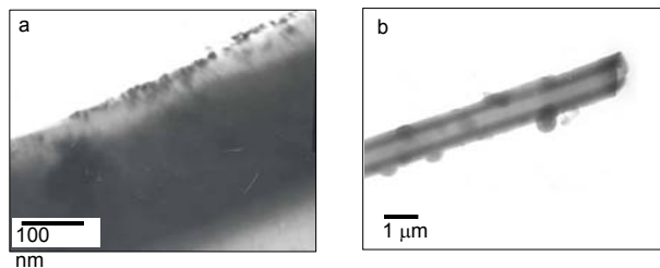
Fig 1. TEM images of citrate-stabilized metal NP anchored onto amine functionalized faceted silica tube (a) Au NP and (b) Ag NP)
