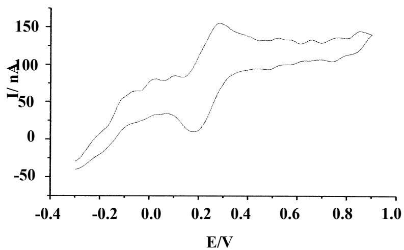
Fig.a: Cyclic voltammogram of \text{TiO}_2 particles anchored with \text{FePO}_3\text{H}_2 , electrolyte \text{KCl} 1M, scan rate 0.1 \text{ V s}^{-1} , reference SCE.
