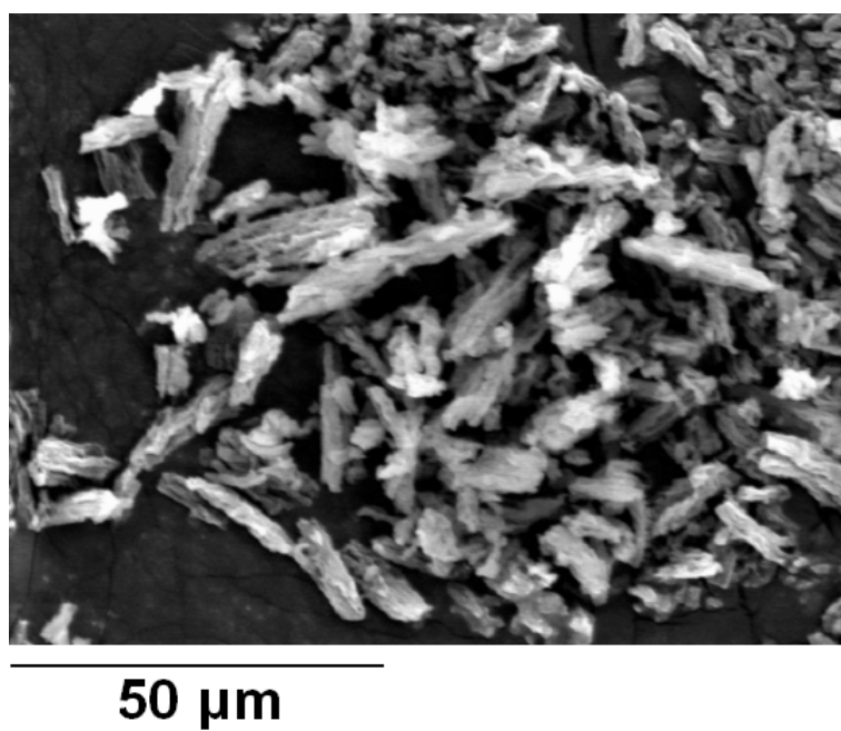
Figure S1: SEM image of a PANI/SBA-15 sample having large particle size.
