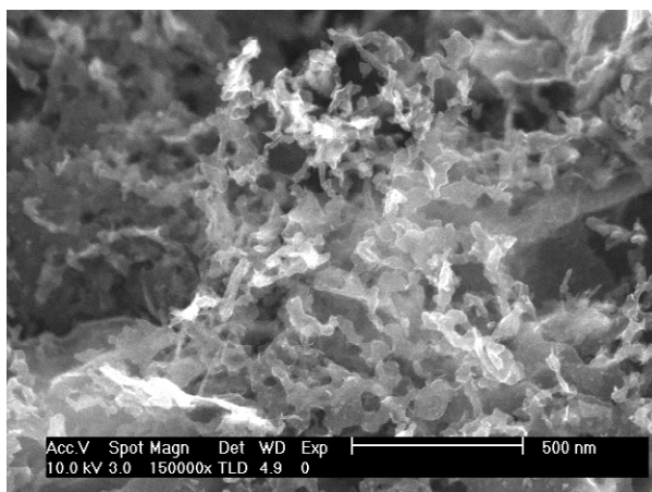
S. 4 SEM image of VN product
