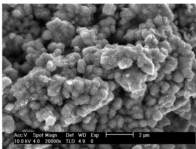
S. 3 SEM image of CrN product.
