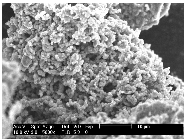
S. 7 SEM image of AlN product.
