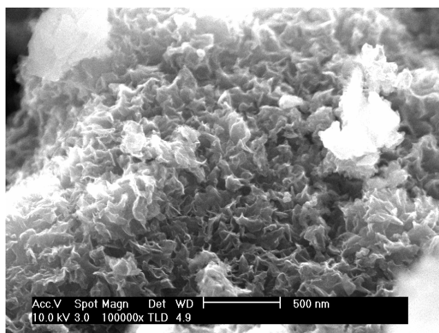
S. 8 SEM image of TiN product
