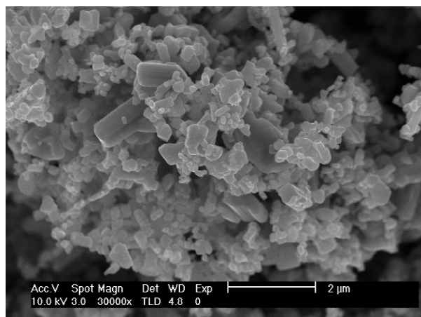
S. 5 SEM image of NbN product.
