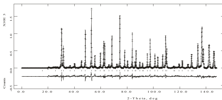
Figure S1. Final profile fit achieved in Fd-3m to the data collected at 2K from RbOs 2 O 6 . Crosses observed data, upper continuous line the calculated profile and lower continuous line the difference. Tick marks show the reflection positions.
