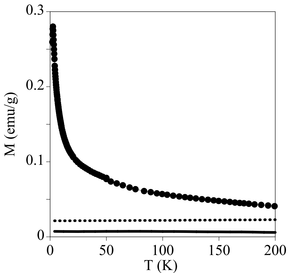
Fig. S1. Temperature dependence of the magnetization for apoferritin-encapsulated Pd nanoparticles (black circles), alkylammonium encapsulated Pd nanoparticles of similar size (dotted line) and bulk Pd (full line). The data for alkylammonium encapsulated Pd nanoparticles have been extracted from reference 7.
