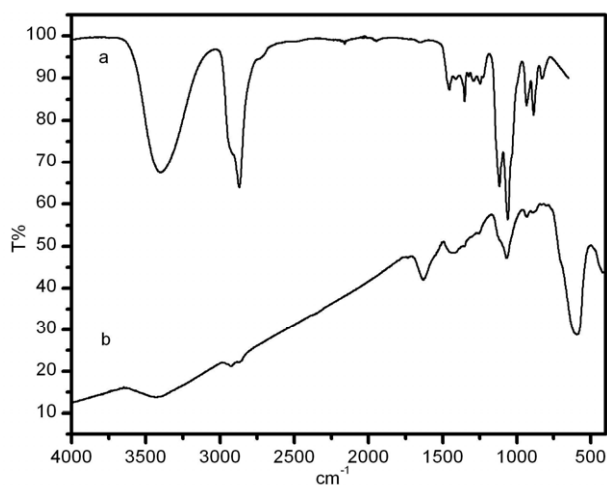
Fig. S2 FT-IR spectra of (a) TREG and (b) as-synthesized Fe 3 O 4 nanoparticles.
