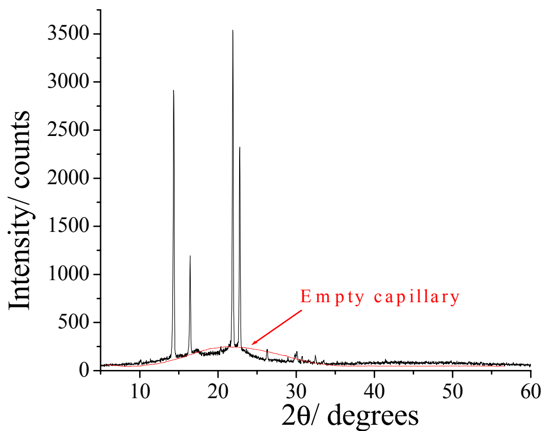
Fig. S1 Powder X-ray diffraction patterns of pure (\text{PEO}_{0.75}\text{G}_{40.25})_6\text{:LiPF}_6 after heat treatment and of an empty capillary.
