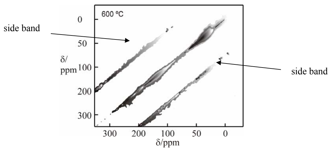
Fig.2. ^{13}\text{C} -RFDR spectrum at 600 °C
