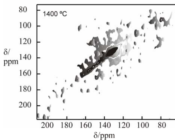
Fig.3. ^{13}\text{C} -RFDR spectrum at 1400 °C
