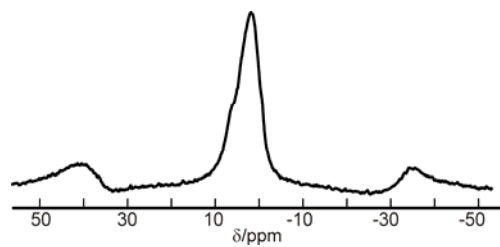
Fig.1. ^1\text{H} spectrum of pre-ceramic \text{SiBN}_3\text{C} at 600 °C, \omega_r / (2\pi) = 14 kHz.
