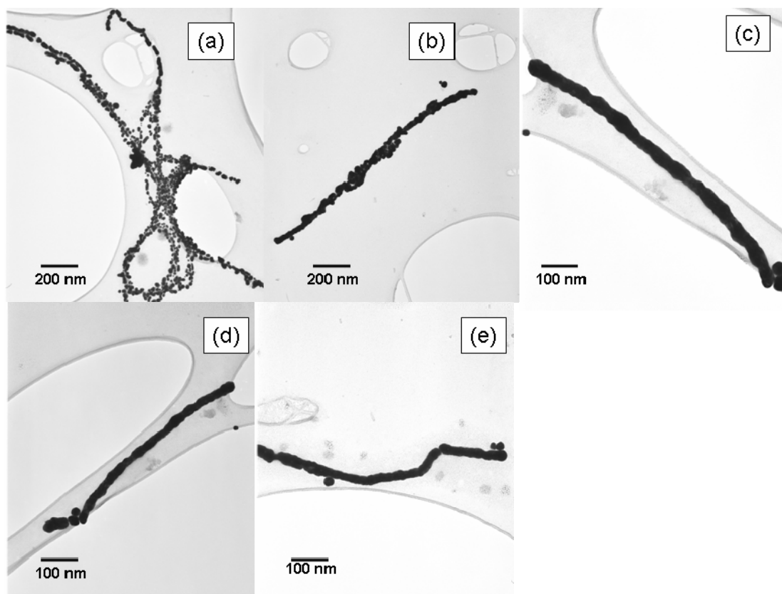
Figure S2. TEM images of metal-CNT hybrids. (a) Ag decorated CNT, (b) Silced CNT with continuous Ag coating, (c) Sliced CNT with continuous Au coating, (d) buckled Ag-CNT, and (e) buckled CNT buckled Au-CNT
