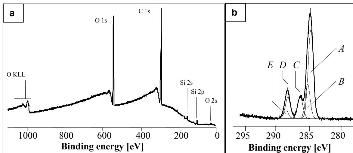
Supporting information 1: (a) XPS wide scan spectrum and (b) C1s core level spectrum of PAA brushes obtained after the hydrolysis of PBA brushes for 1.5 h.
