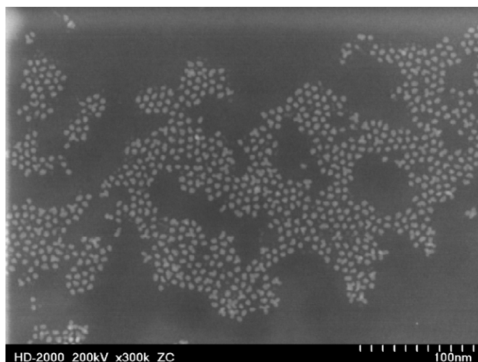
Supporting 1. TEM image of the CdSe/TOPO QDs with a band-edge absorption at 588 nm and a mean core diameter of 4.5 \pm 0.3 nm as determined by TEM.
