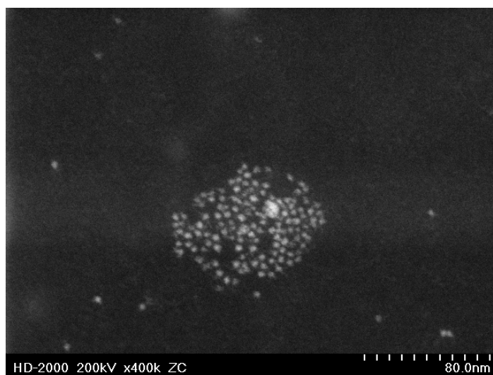
Supporting 2. TEM image of the PbS/OA QDs with a band-edge absorption at 1108 nm and a mean core diameter of 3.5 \pm 0.5 nm as determined by TEM.
