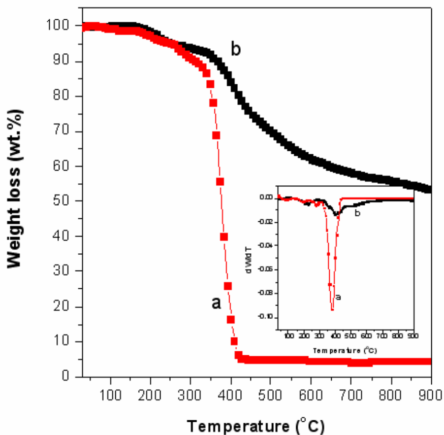
Figure S1. TGA and DTG curves (inset) of (a) PEO- b -PMMA diblock copolymer and (b) as-made mesoporous carbon FDU-18 conducted in N 2 atmosphere.
