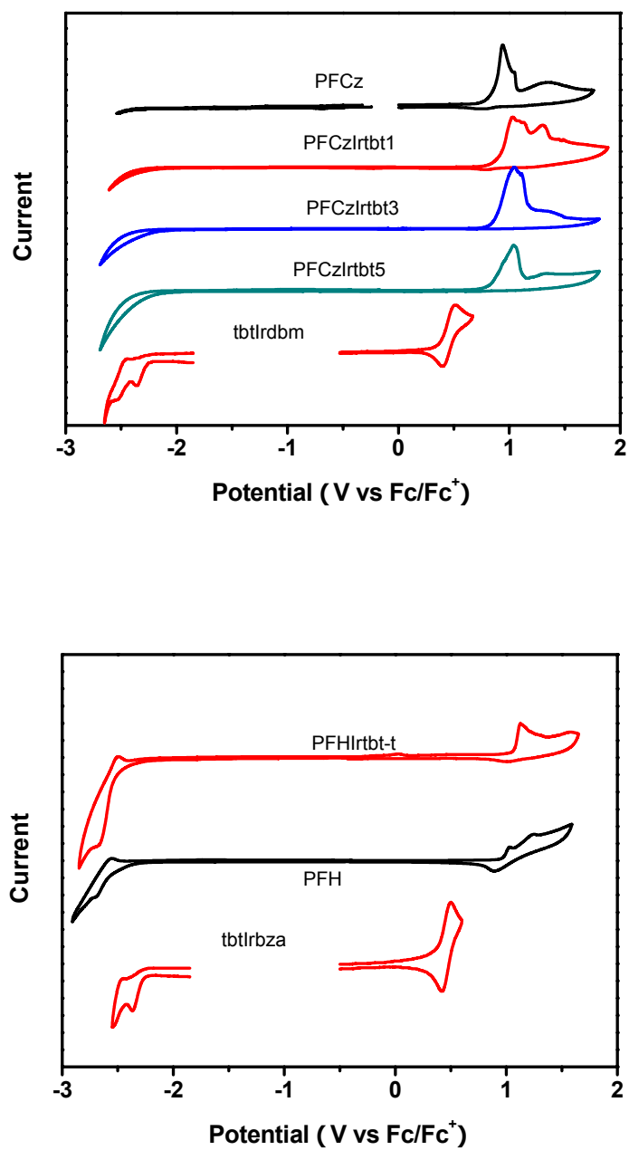
Figure S2. Cyclic voltammograms of PFCz, PFH, P1-4 and corresponding iridium complexes.
