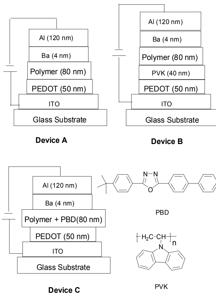
Figure S3. The configurations of the Device A, B and C, along with the molecular structures of materials.
