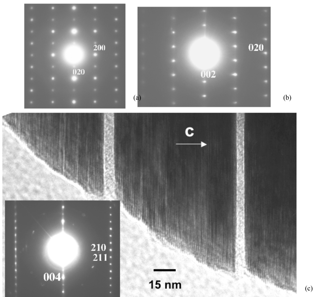
Figure S1: HTiNbO 5 mother structure : (a) [001] and (b) [100] SAED patterns. (c) overall [1 \bar{2} 0] HREM image and ED pattern.
